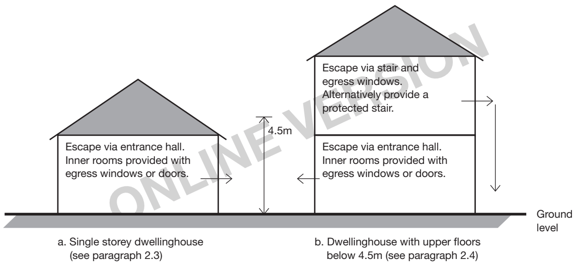
Diagram 1 Means of escape from dwellinghouses
